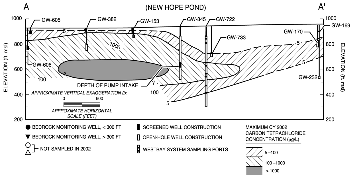
Fig. 6.21. Maximum carbon tetrachloride concentrations in Maynardville Limestone at depths between 200 and 500 ft.
