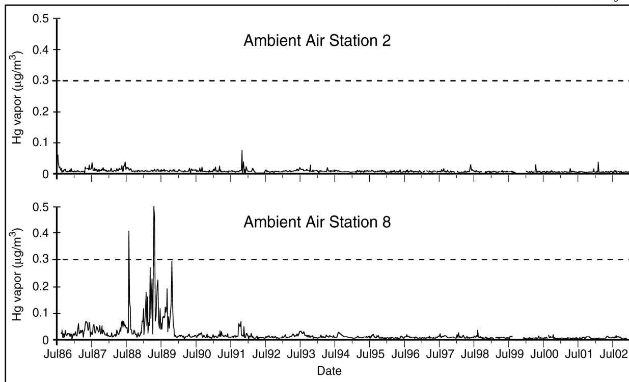
Fig. 6.4. Temporal trends in mercury vapor concentration for the two active airborne mercury monitoring sites at the Oak Ridge Y-12 Complex, July 1986 through July 2002. The dashed line represents the EPA reference concentration of 0.3 \mu\text{g}/\text{m}^3 .
