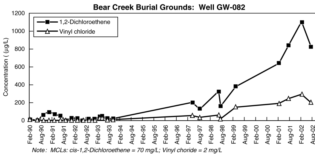
Fig. 6.25. Volatile organic compound concentrations in Bear Creek Burial Grounds Wells GW-627, GW-653, and GW-082.
