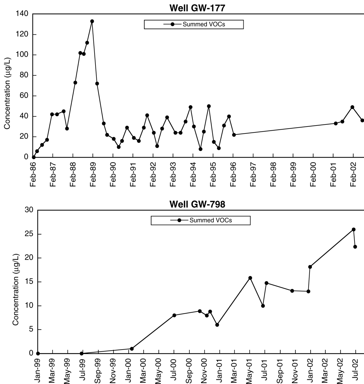
Fig. 6.28. Summed VOC concentrations in Wells GW-177 and GW-798.
