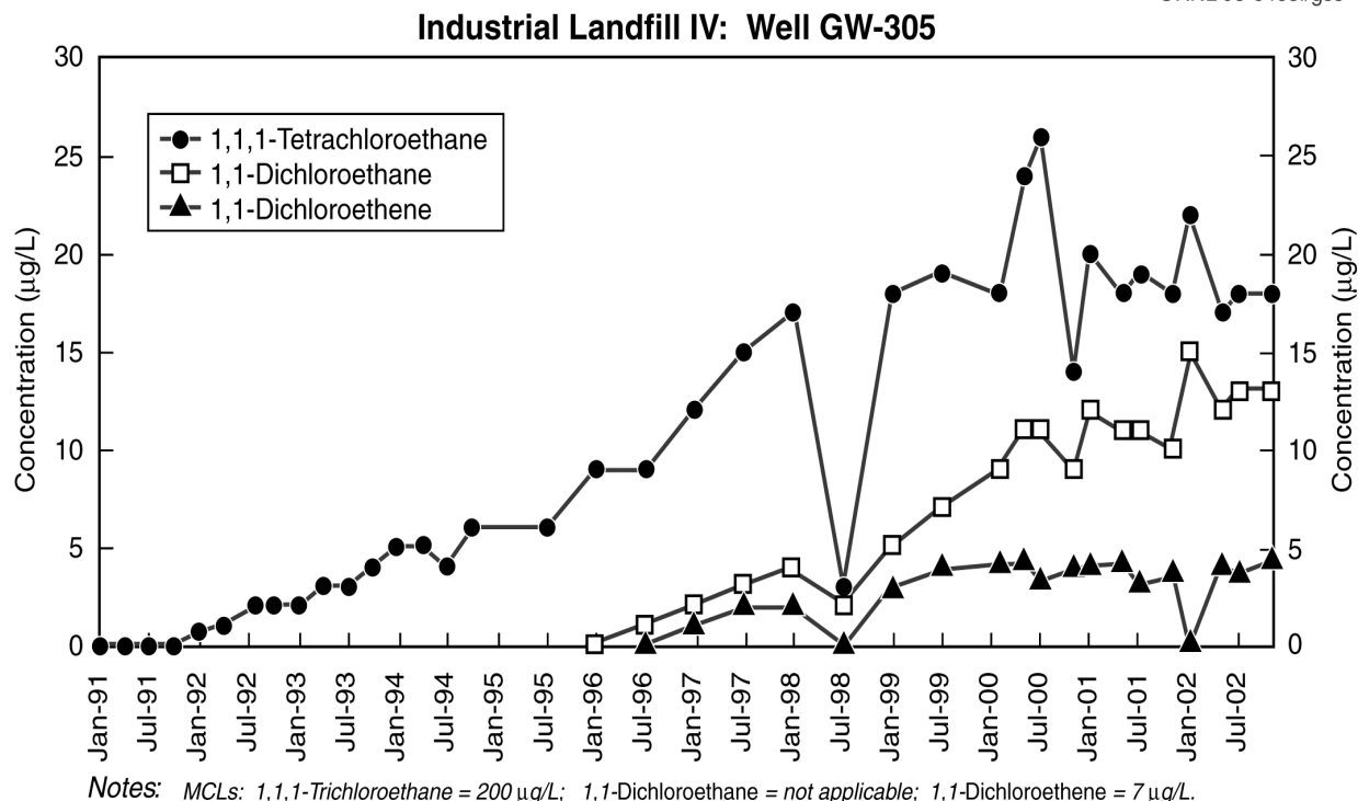
Fig. 6.29. Volatile organic compound concentrations in Industrial Landfill IV Well GW-305.
