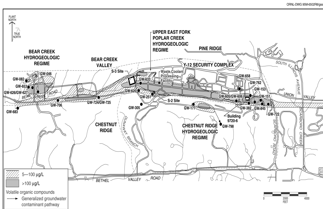
Fig. 6.18. Summed volatile organic compounds in groundwater at the Y-12 Complex.
