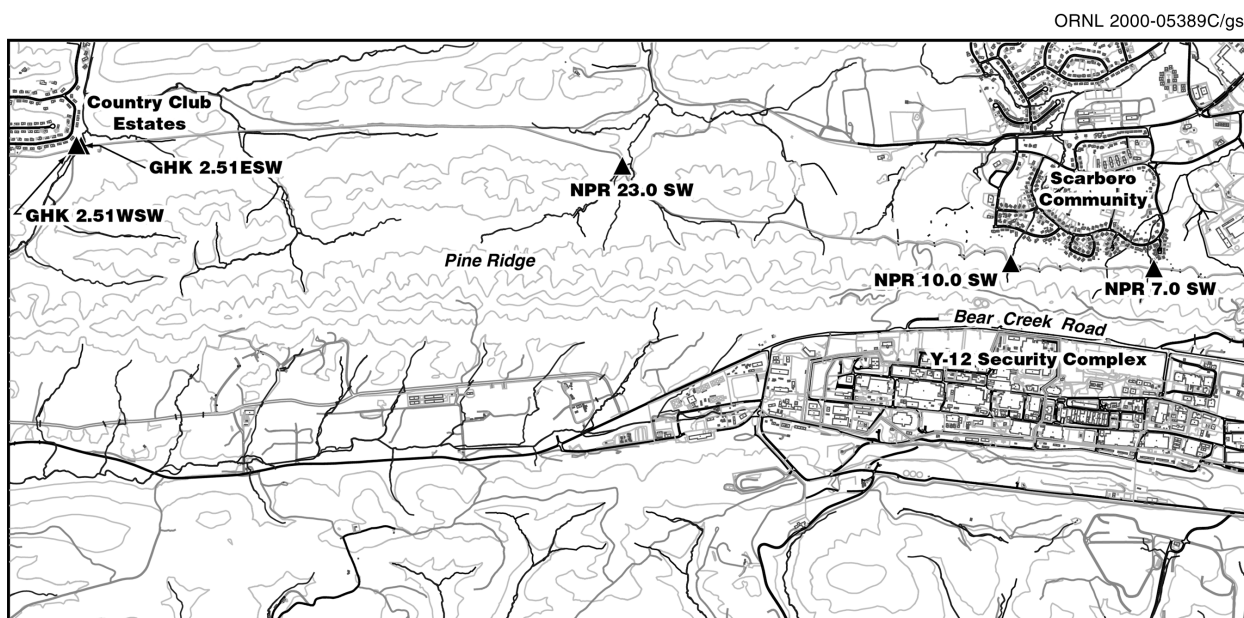
Fig. 6.24. Surface water sampling locations north of Pine Ridge (NPR), 2002. (GHK = Gum Hollow kilometer.)
