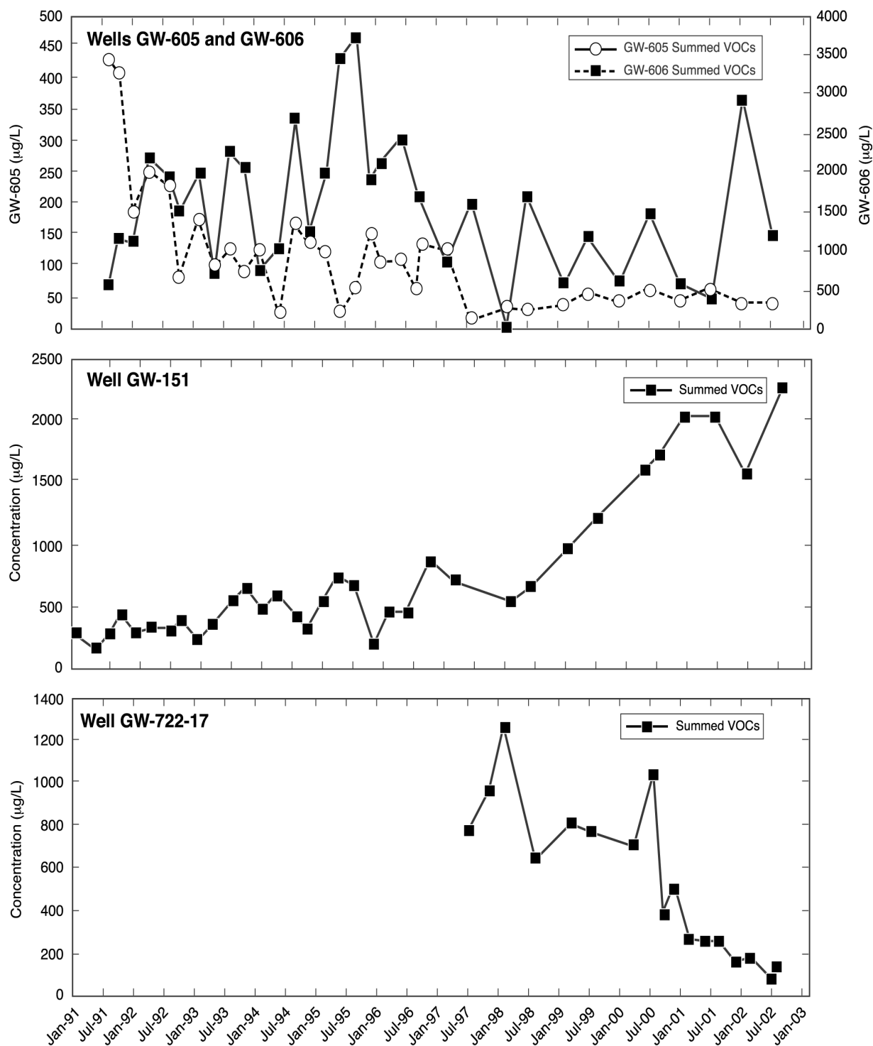
Fig. 6.20. Summed volatile organic compound concentrations in selected wells near New Hope Pond and exit pathway wells.
