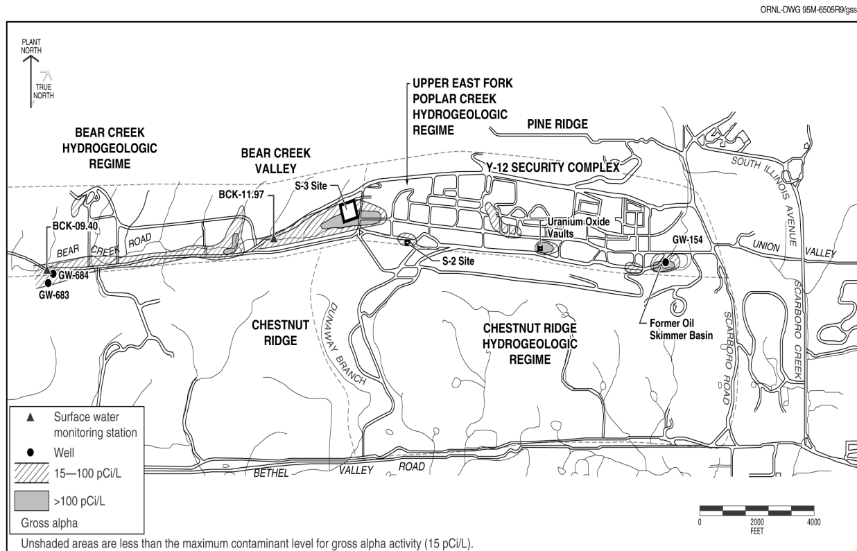
Fig. 6.22. Gross alpha activity in groundwater at the Y-12 Complex.
