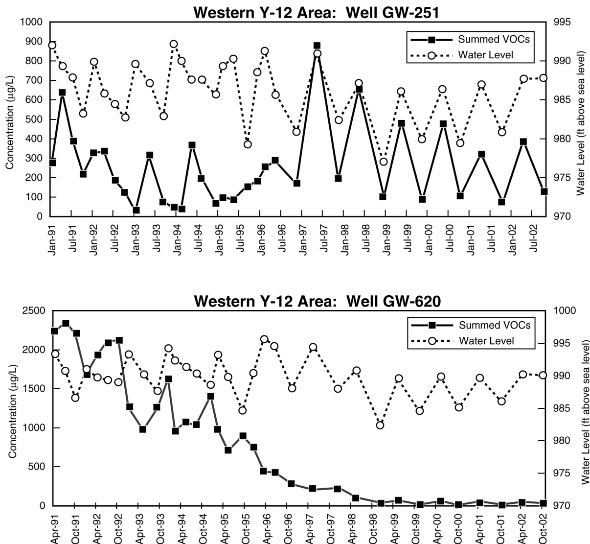
Fig. 6.19. Volatile organic compound concentrations in groundwater in selected wells near source areas in the Upper East Fork Poplar Creek Hydrogeologic Regime.
