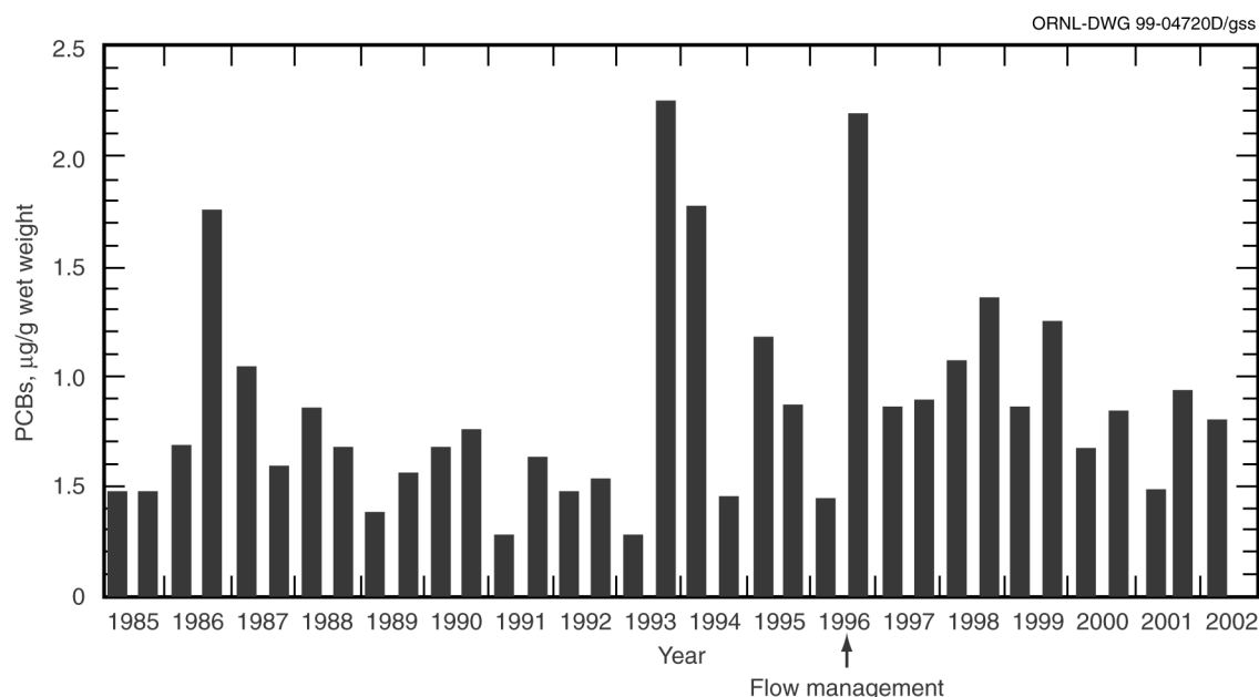
Fig. 6.9. Mean concentrations of PCBs in redbreast sunfish muscle fillets in East Fork Poplar Creek at Station 17 through spring 2002.
