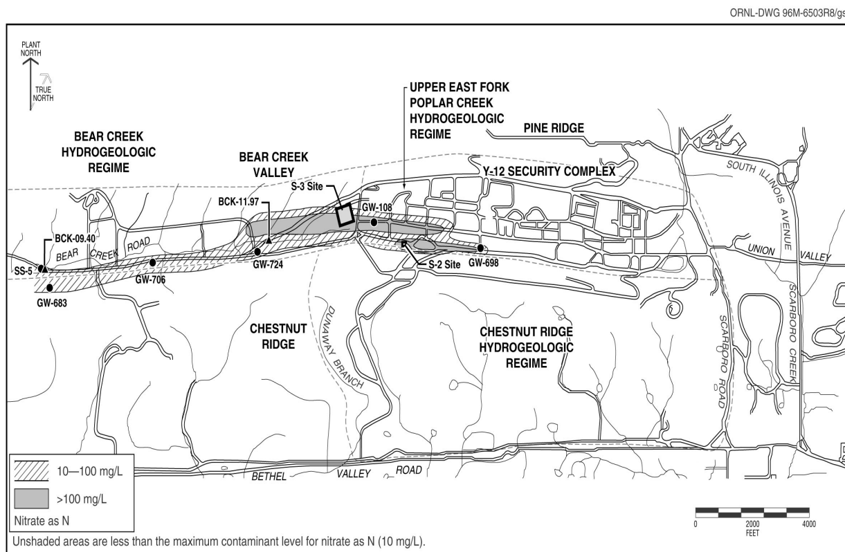
Fig. 6.17. Nitrate (as N) observed in groundwater at the Y-12 Complex.
