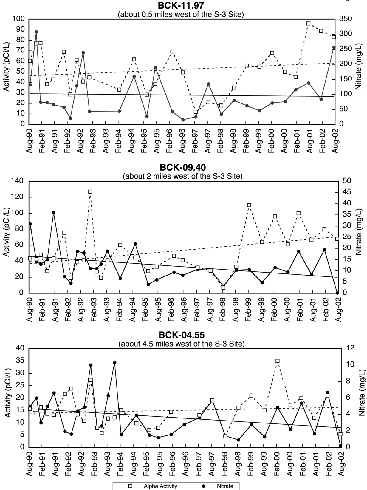
Fig. 6.27. Concentrations of selected groundwater contaminants in Bear Creek.
