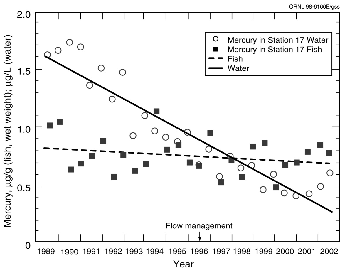
Fig. 6.8. Semiannual average mercury concentrations in muscle fillets of redbreast sunfish and water in East Fork Poplar Creek at Station 17 through spring 2002.
