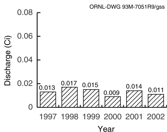
Fig. 6.1. Total curies of uranium discharged from the Y-12 Complex to the atmosphere, 1997–2002.
