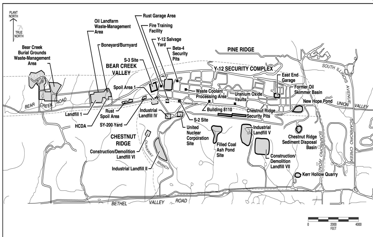
Fig. 6.14. Known or potential contaminant sources for which groundwater monitoring was performed during CY 2002.
