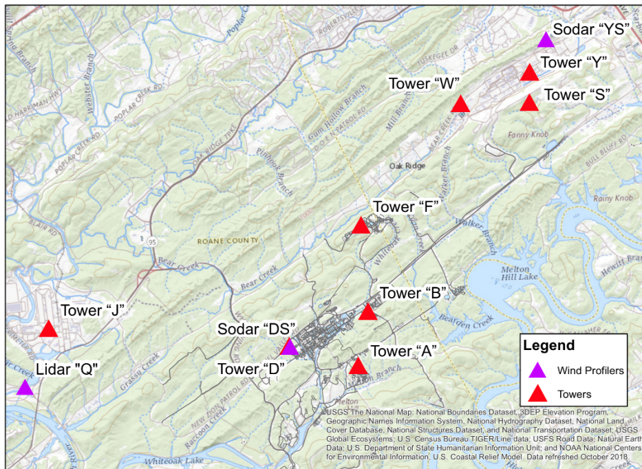
Fig. 3.1. Oak Ridge Reservation meteorological tower, sonic detection and ranging (SODAR), and light detection and ranging (LIDAR) device locations.
