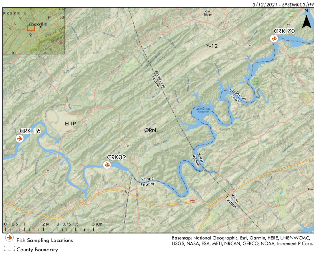
Fig. 5.4. Oak Ridge Reservation fish sampling locations.
