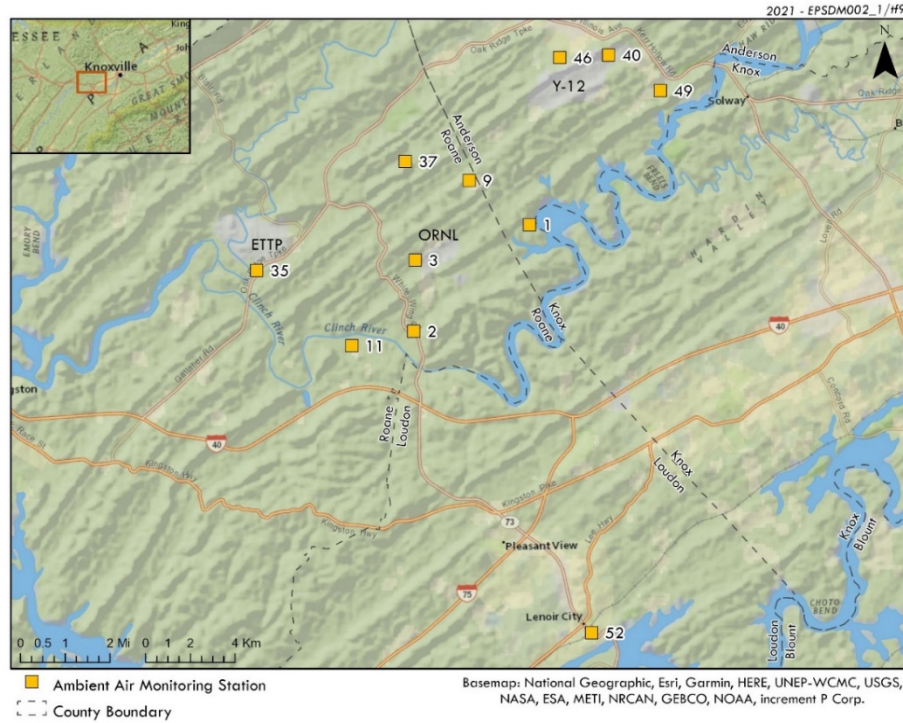
Fig. 5.1. Oak Ridge Reservation perimeter ambient air monitoring stations.
