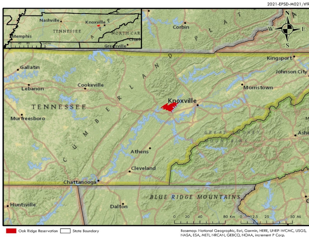
Fig. 2.1. Location of the Oak Ridge Reservation.
