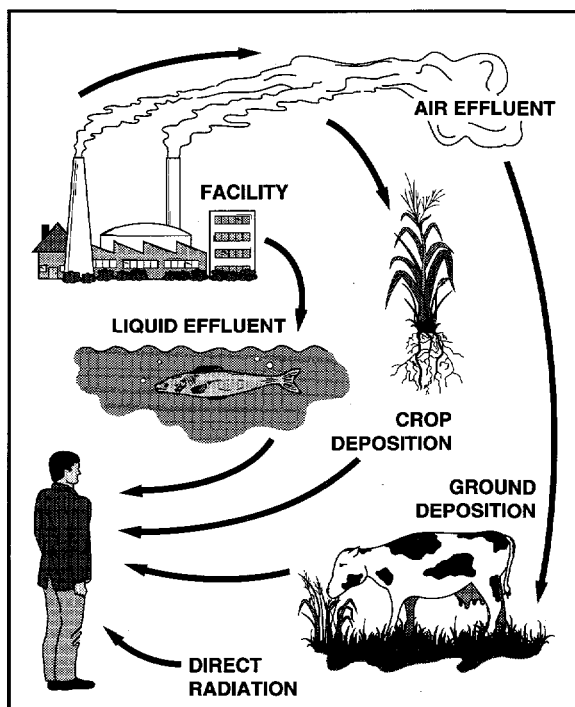
Fig. 12. Chemical and radiation pathways. We can receive internal or external exposure to chemicals, radioactive materials, and radiation by way of a number of pathways. We receive radiation directly from cosmic radiation and from particles embedded in soil and suspended in air and water. We can breathe air or drink water that have both chemical and radiological airborne contaminants suspended in them. In addition, airborne contaminants that settle on grass in pastures and hayfields can be eaten by cows, and the contaminants can show up in the milk we drink. Similarly, contaminants can be retained in honey, fish, and game animals.
