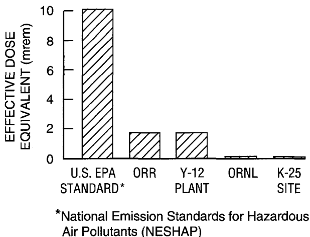
Fig. 13. Total 1994 effective dose equivalents to maximally exposed individual from airborne releases. In comparison, local natural background radiation is about 300 mrem (3 mSv) per year.
