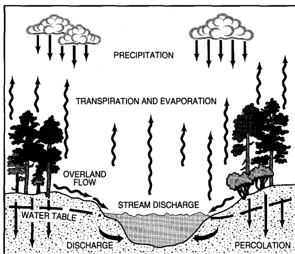
Fig. 16. Groundwater is precipitation that has percolated into subsurface rock and soil. The water table, the depth to which the ground is saturated with water, varies seasonally with the precipitation rate. Groundwater moves through the ground and discharges to bodies of surface water where the two meet. Because groundwater can transport both chemical and radiological pollutants from underground waste-burial sites, both surface water and groundwater are sampled on and off the reservation to determine the presence, amount, and movement of wastes.
