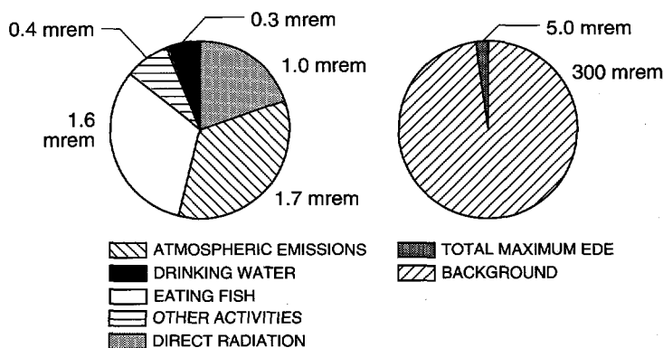
Fig. 20. A comparison of maximum EDEs via various exposure pathways.
